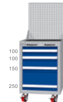
EA-7042MA W566xD640xH1380
