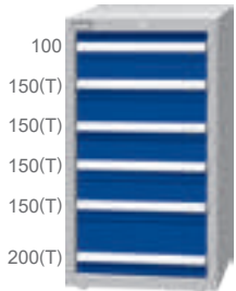
EA-10062(T) W566xD607xH1000
