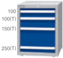
EA-7042(T) W566xD607xH700
