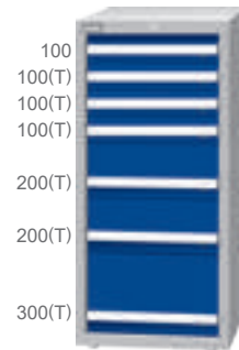
EA-12074(T) W566xD607xH1200
