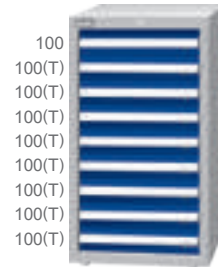
EA-10091(T) W566xD607xH1000
