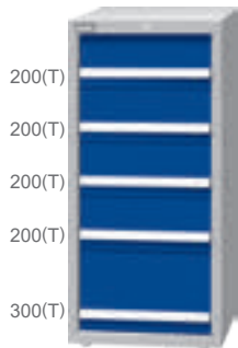
EA-12052(T) W566xD607xH1200
