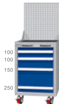
EA-7042MA W566xD640xH1380
