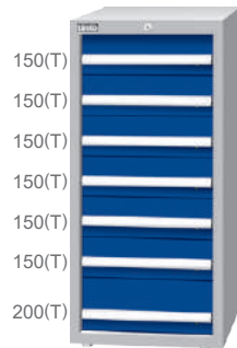
EA-12071(T) W566xD607xH1200 EB-12071(T) W718xD607xH1200 ED-12071(T) W718xD759xH1200
