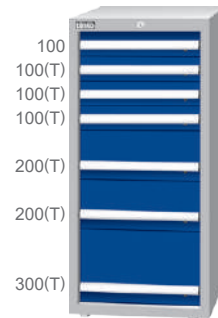
EA-12074(T) W566xD607xH1200 EB-12074(T) W718xD607xH1200 ED-12074(T) W718xD759xH1200
